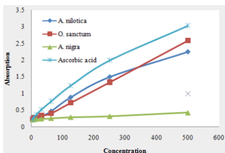
Figure 1: Ferric reducing power increases with the increasing concentration of the sample, concentration in µg/mL.
